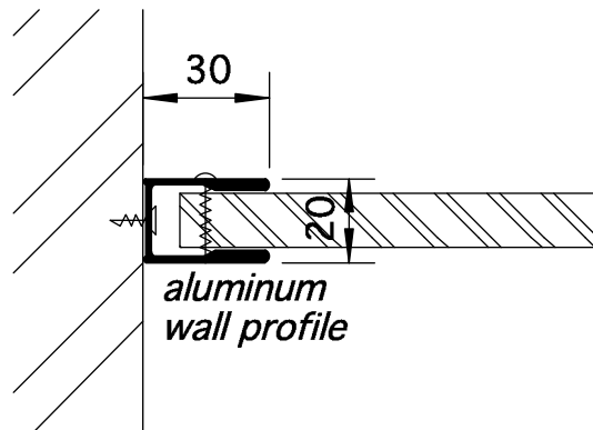
connection intermediate panel/front wall
