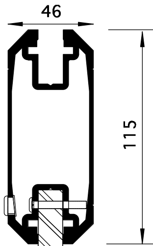
aluminum stabilisation profile
